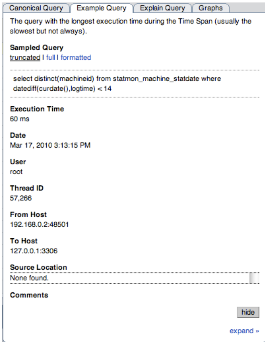
Figure 3.7 MySQL Enterprise Monitor User Interface: Example Query Tab for a Query
