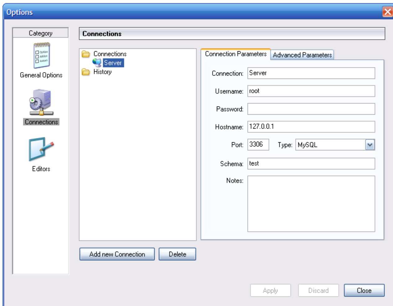
Figure 21.2. Options Dialog: Connections
