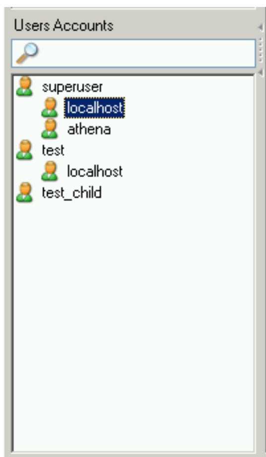
Figure 13.1. User Accounts
