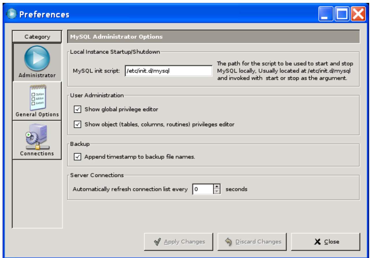
Figure 21.1. Options Dialog
